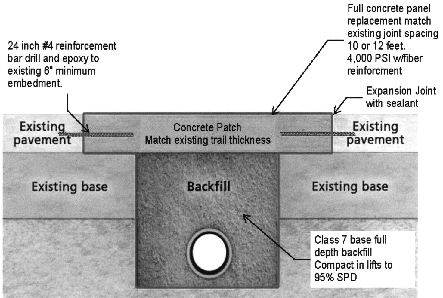
Figure 4 - Trail Patch Detail
