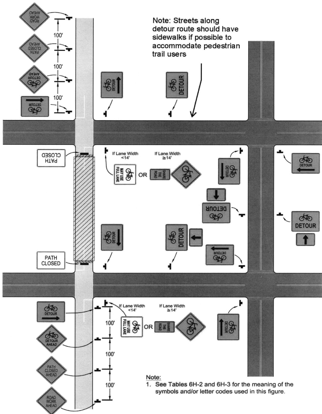
Figure 3 - Temporary On-Road Detour for Shared Use Paved Trail
