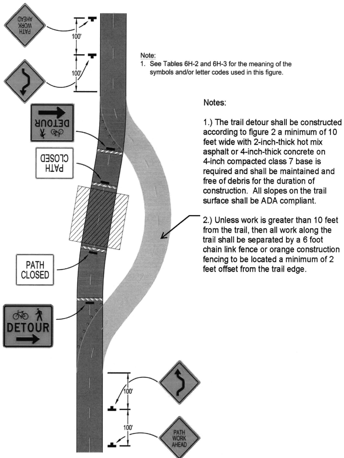
Typical Application B3
