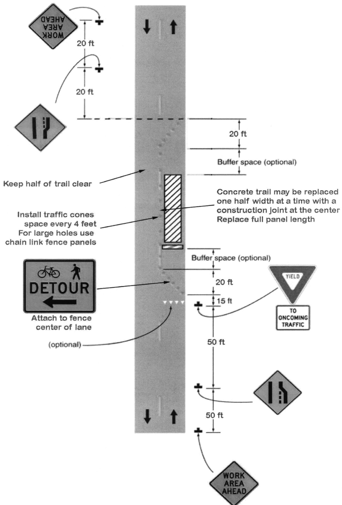
Figure 1 - One Lane Trail Closure
